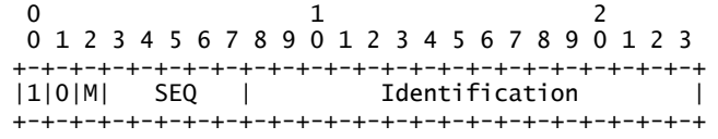
Fig. 2: L2 fragmentation header in NDN-RIOT
