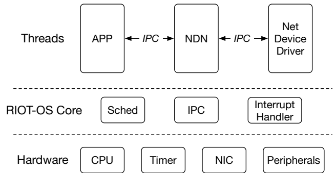
Fig. 1: Software architecture of NDN-RIOT
